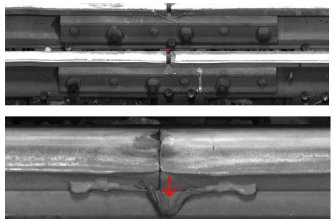
View of the Rails as Provided by Joint Bar Video Inspection System. Overview (Upper Image) and Detail With Crack (Lower Image).
